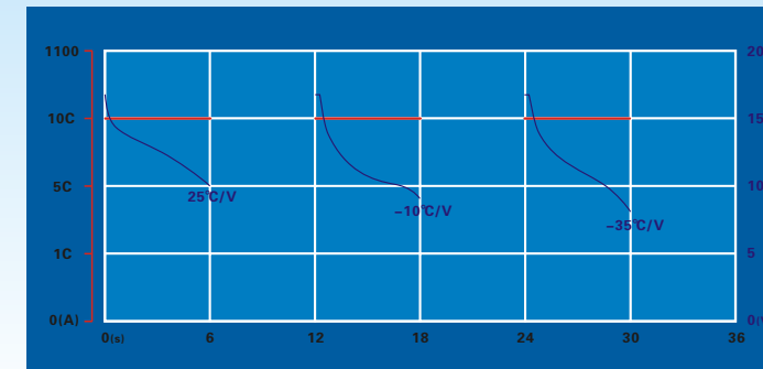
LP類電池不同環境溫度下瞬間放電特性曲線圖 ▲ Transient discharge characteristic curves of LP battery under different environment temperature
