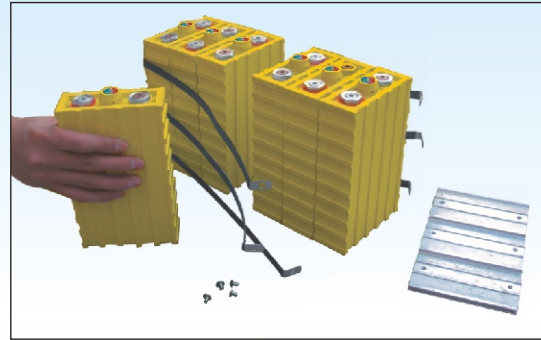
拆開拉條，更換同容量電池 Release the straps and replace the cell with same capacity
