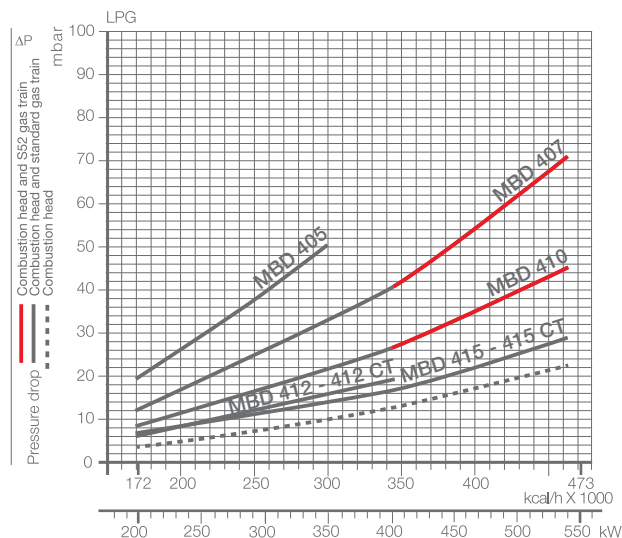
RS 44/M MZ (LPG)
