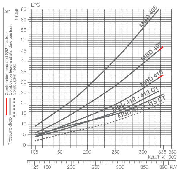
RS 34/M MZ (LPG)
