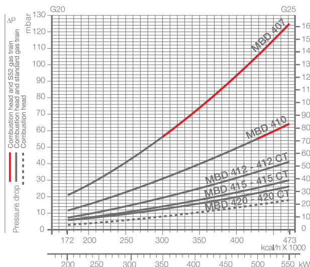
RS 44/M MZ (NATURAL GAS)
