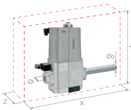
Example of gas train "MULTIBLOC" type MBC 1200
