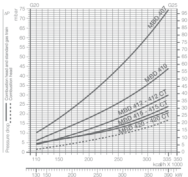
RS 34/M MZ (NATURAL GAS)
