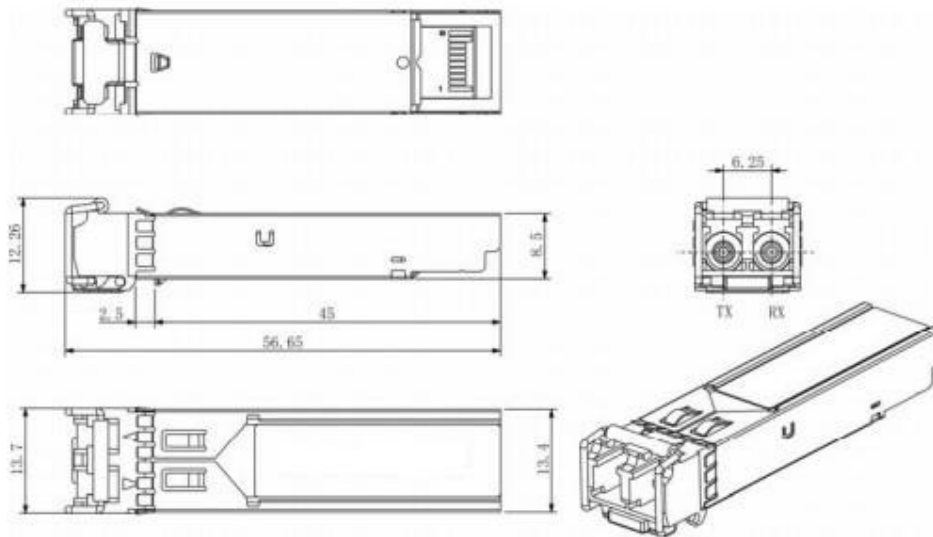
Mechanical Drawing
