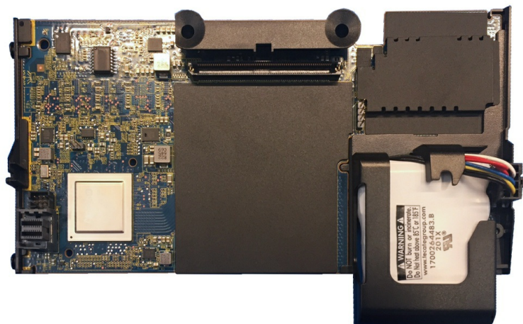
Figure 4. ThinkSystem RAID 930-4i-2GB 2 Drive Adapter Kit for SN550 (included heatsink not shown)
