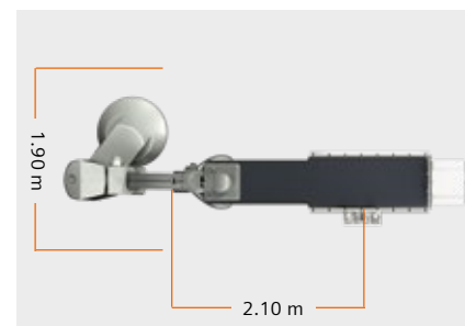
Ceiling-like coverage of 2.10 m along and 1.90 m across the table on a floor-mounted system
