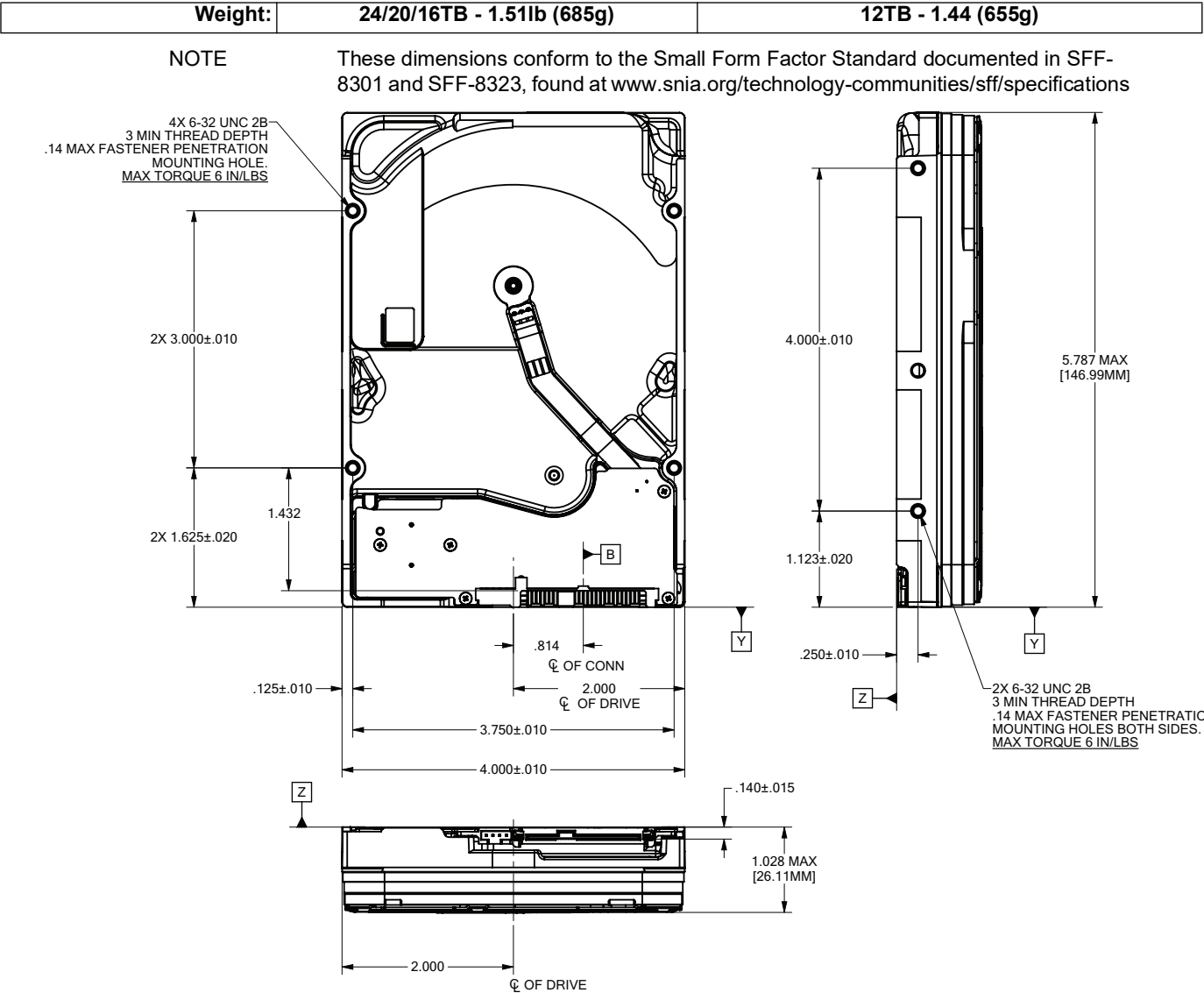
Figure 4. Mounting configuration dimensions NOTE The image is for mechanical dimension reference only and may not represent the actual drive.
