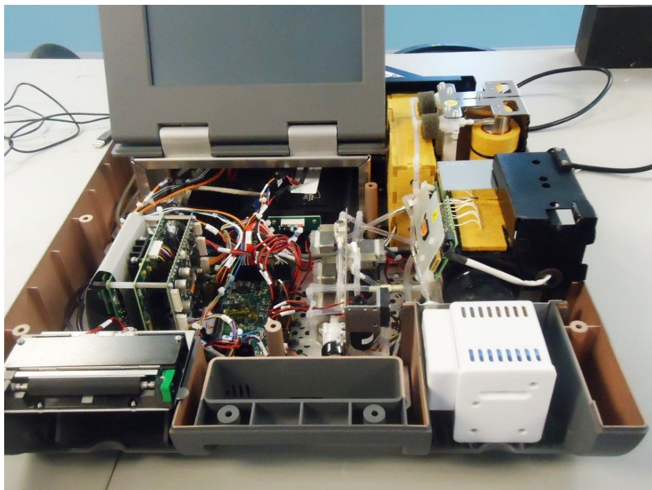
Internal View
