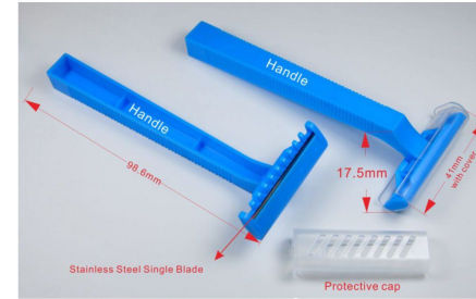
FY0913 - 1S (Stainless steel single blade)
