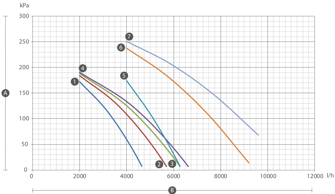
Useful head system (Q/N)
