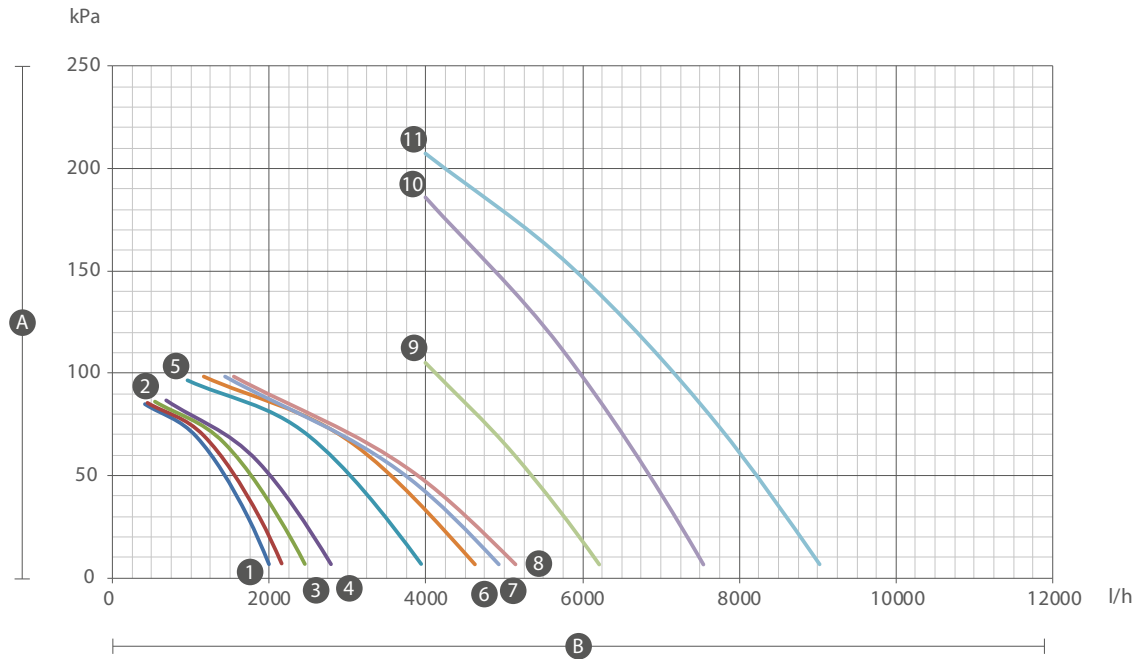
Useful head system (P/A)
