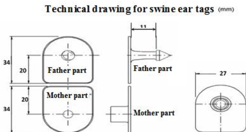
Fig.3 Technical drawing for swine ear tags
