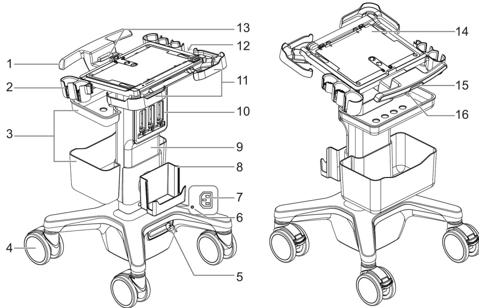
Figure B-1 Overview of the Trolley
