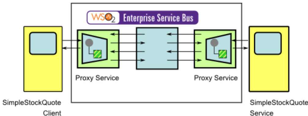
Figure 2: Example Scenario of the Messaging Gateway EIP
