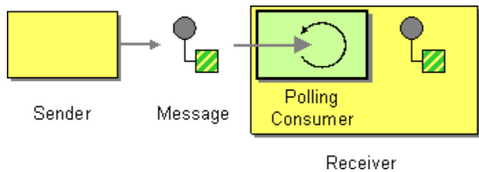
Figure 1: Polling Consumer EIP
