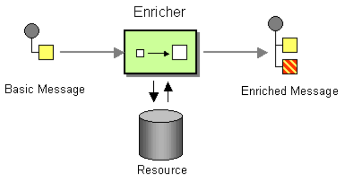
Figure 1: Content Enricher EIP
