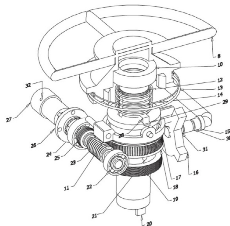
Gear Machanism
