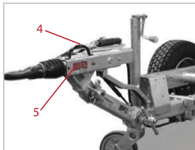
4 - Electrical Connection Socket 5 - Safety break arm
