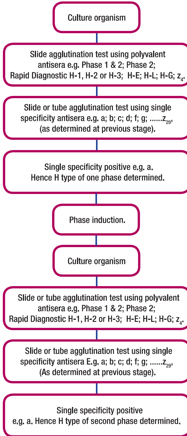
Figure 2 - Summary of Salmonella H-Typing Procedures
