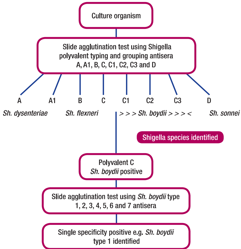
Figure 1 - Summary of Shigella Sero-grouping and Typing Procedures
