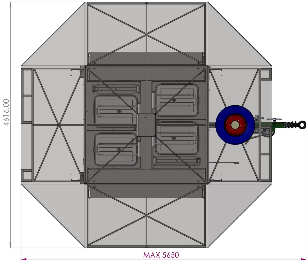
Fig.8 Dimensions of Mobile Field Kitchen
