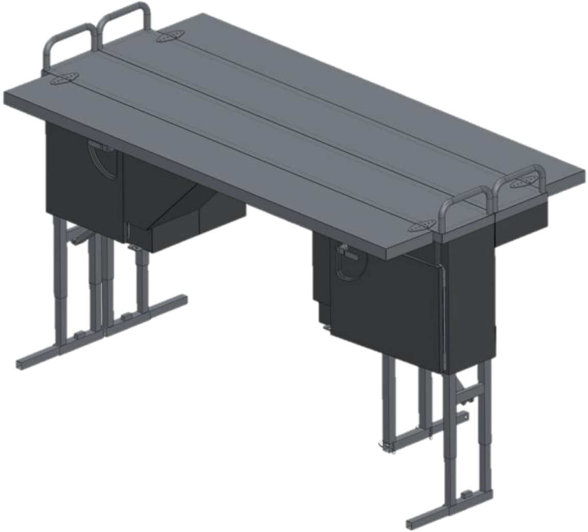
Fig.41 Mounted Service Module
