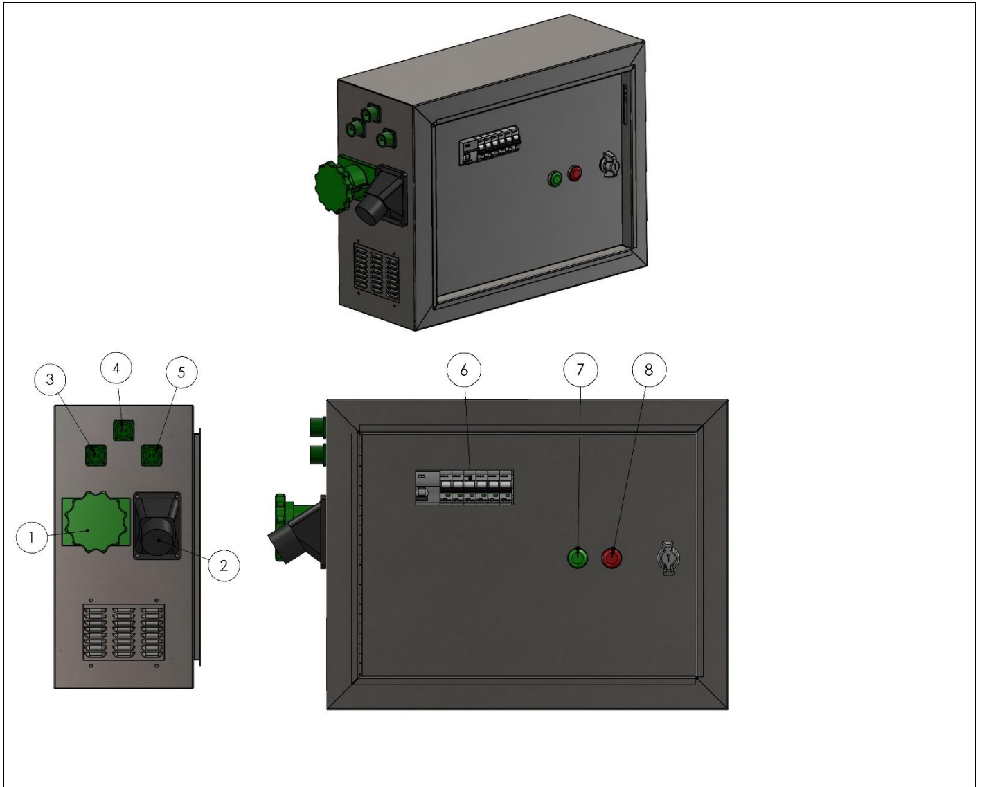
Fig.49 Electrical Plant
