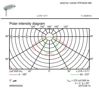
OFPC1_SGS102 1xSON-TTP250W MR.EPS
