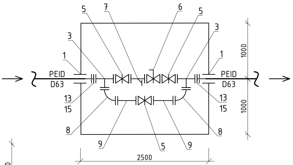
Camin F/RP-2 2500x2000
