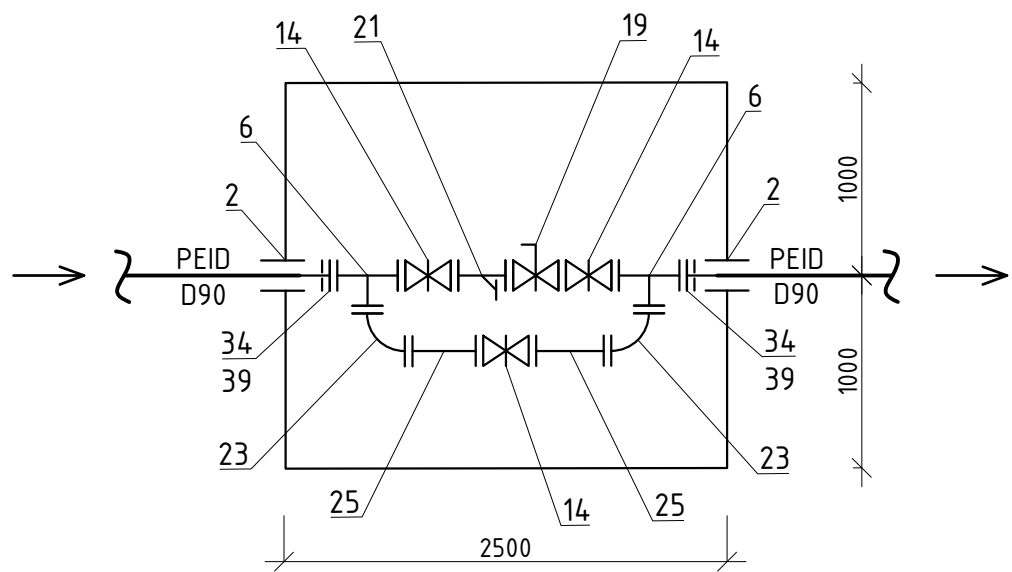
Camin F/RP-1 2500x2000
