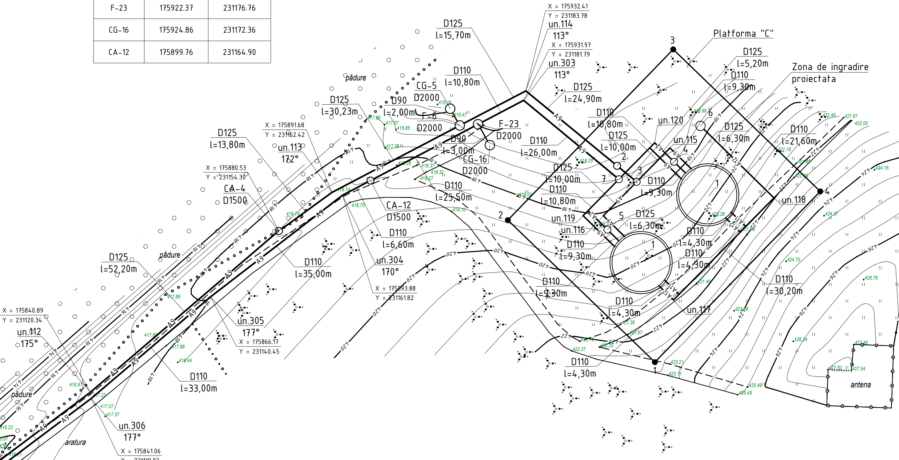
EXPLICATIA CONSTRUCTIILOR PLATFORMA "C" cota 0.000 = 420.000
