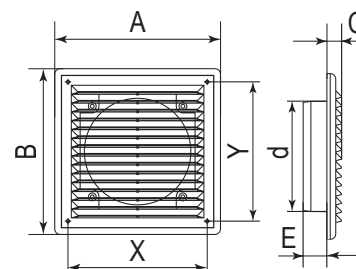
Overall dimensions
