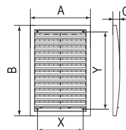
Overall dimensions
