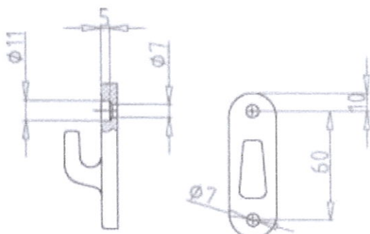
Figure no. 1 (cast iron element top)
