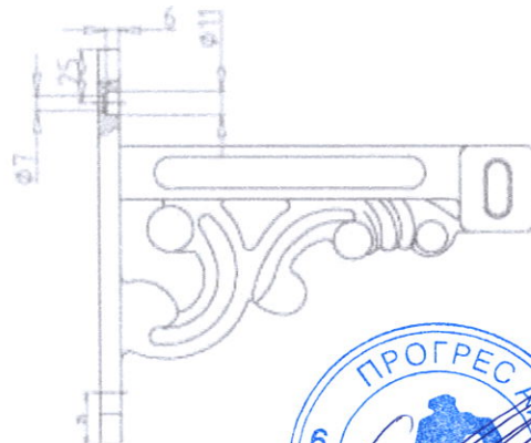
Figure no. 2 (cast iron element bottom)
