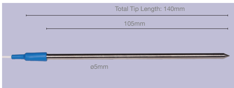
ST100T - Long Tipped Sensor Probe
