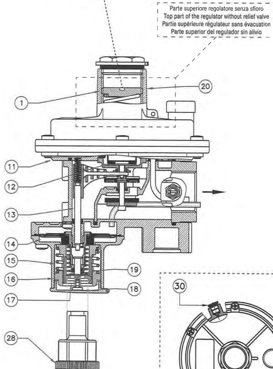
fig. 2b - STANDARD 2MB DN 15 - DN 20 - DN 25 (Q max = 120 Nm³/gas)
