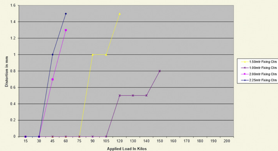
T60 Weight Test Across Track - Measuring Distortion
