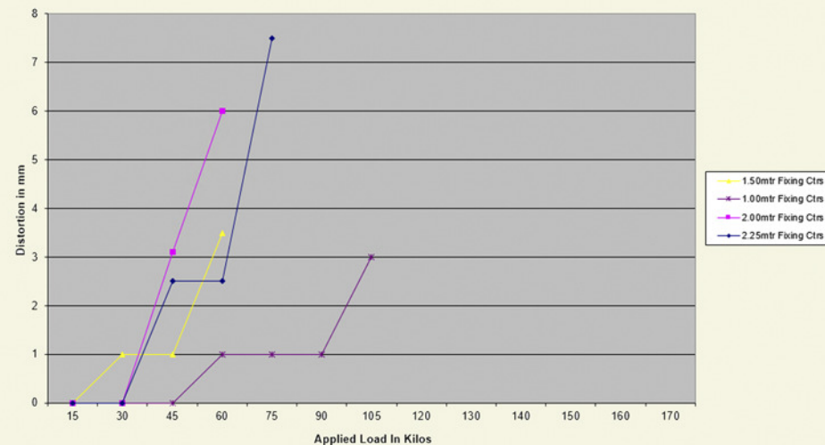
T60 Weight Test Across Joint - Measuring Distortion
