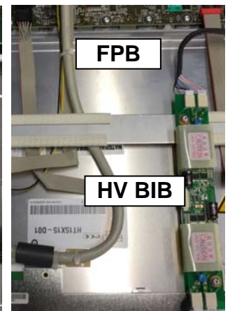
Fig. 3: FPB for HV BIB
