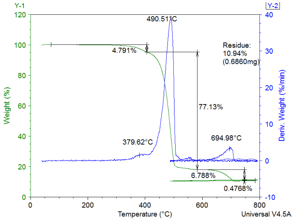
Fig.4 TGA curve of original sample
