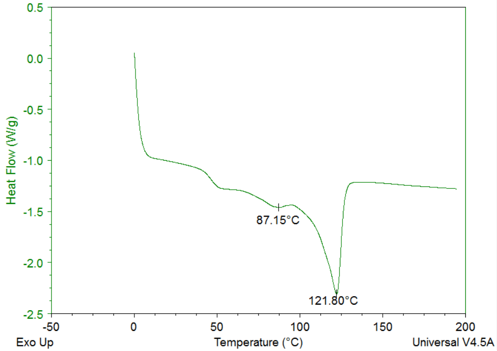
Fig.5 DSC curve of original sample
