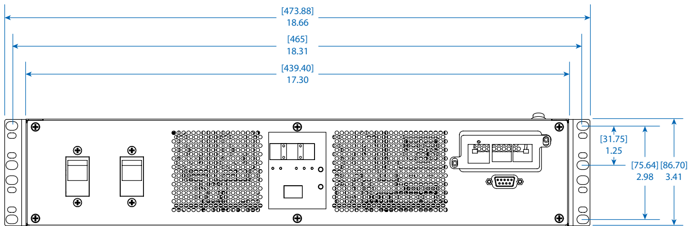
FRONT VIEW
