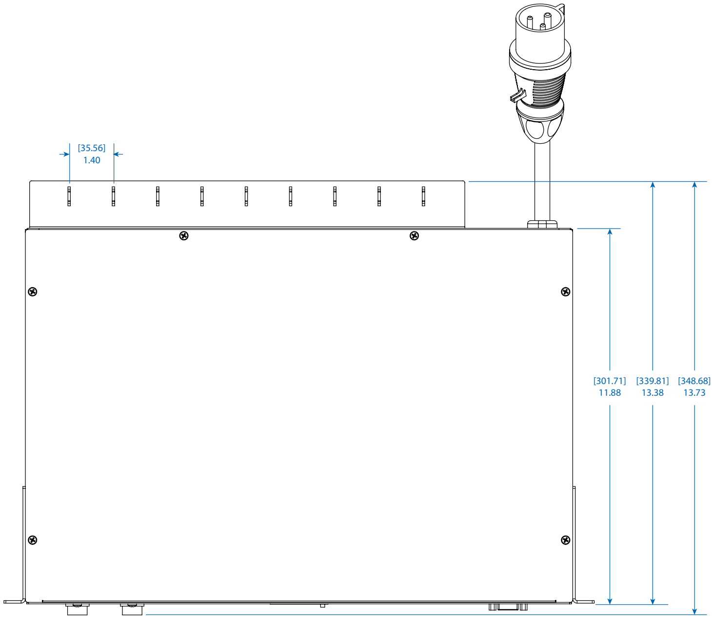
TOP VIEW
