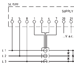
Q52D3L063X4C2 - Q52D3L125X4C2 system 3 fazowy, 3 przewodowy for three-phase three wires system
