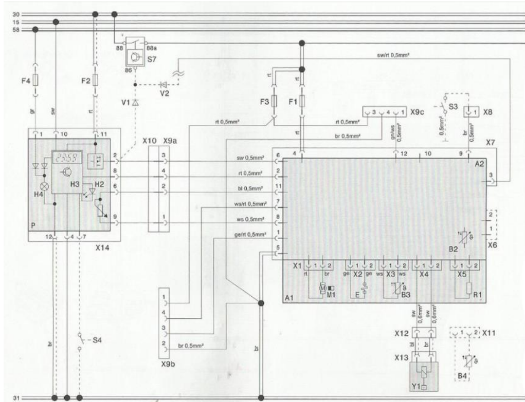
Drawing No.4: Circuit Diagram
