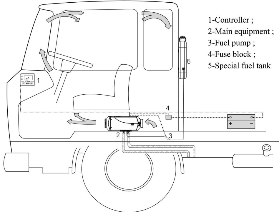
Drawing No.7: Installation drawing
