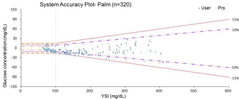
Figure 8 Bias analysis (mg/dL)
