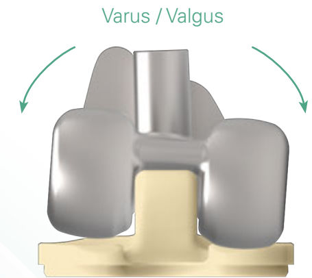
Varus/valgus lift-off is limited to ±1.4° for increased stability
