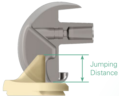
Jump height distance is 21.4 mm to reduce potential for dislocation
