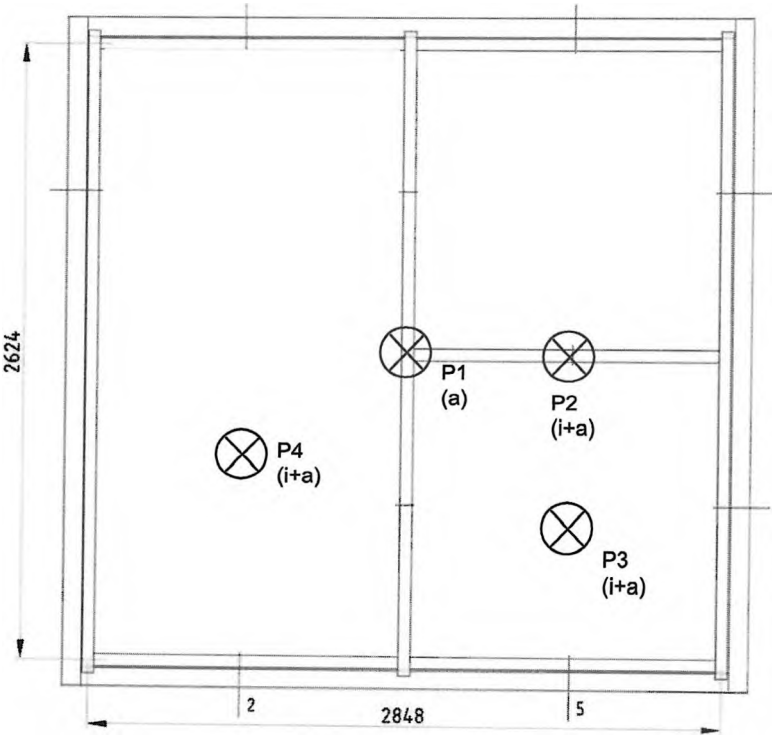
Illustration 2 Impact loads
