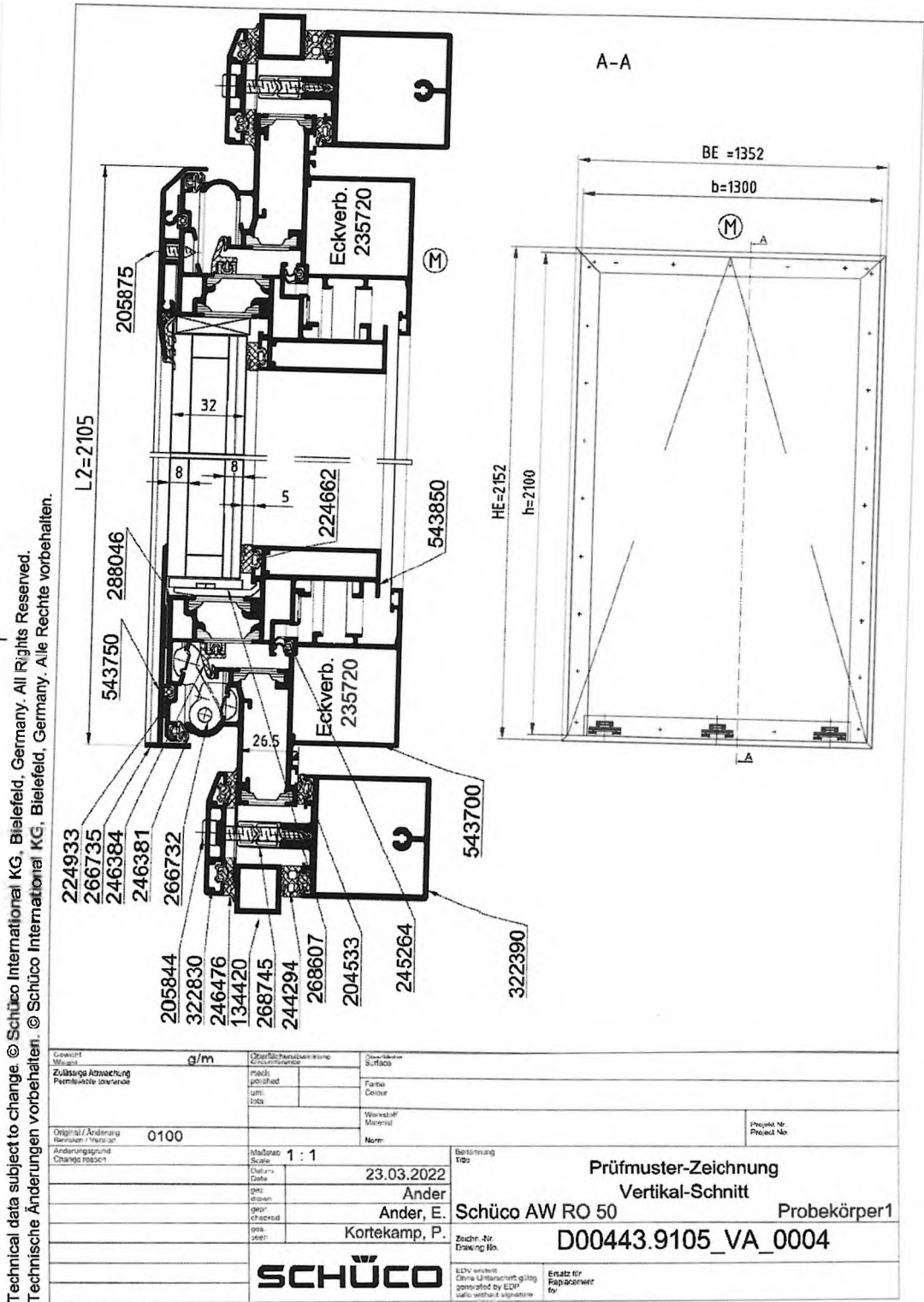
Picture 4 Vertical section
