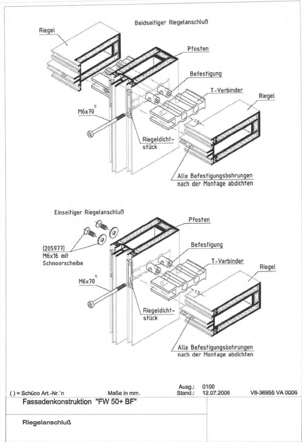
Drawing 7 Stick construction
