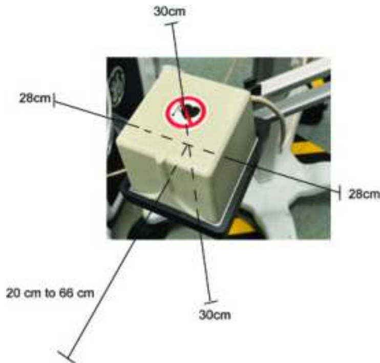
Figure 5-27 • Magnetic Field Range from the Transmitter
