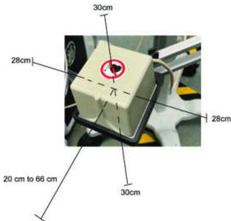
Figure 13-135 • Magnetic Field Range from the Transmitter
