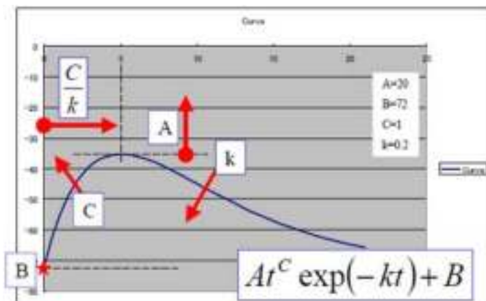
Figure 13-42 • Gamma Curve
