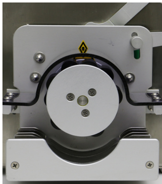
Pumphead open
