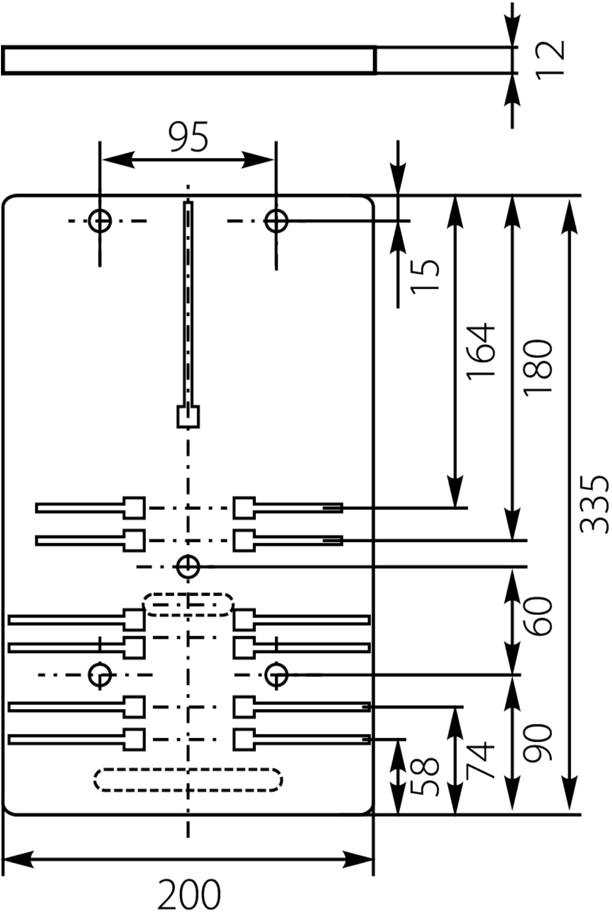
Meter board T-U 1F/3F-b/z-12 Universal, without protections, IP20
