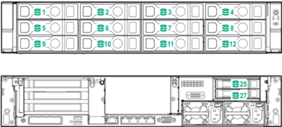
12 LFF + 2 rear SFF drives
