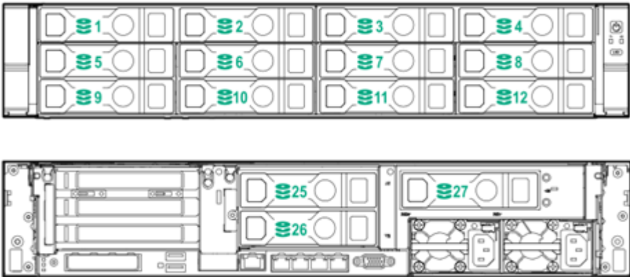
12 LFF + 3 rear LFF drives
