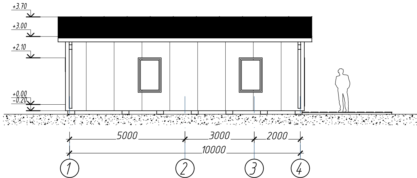
Fatada 1-4
