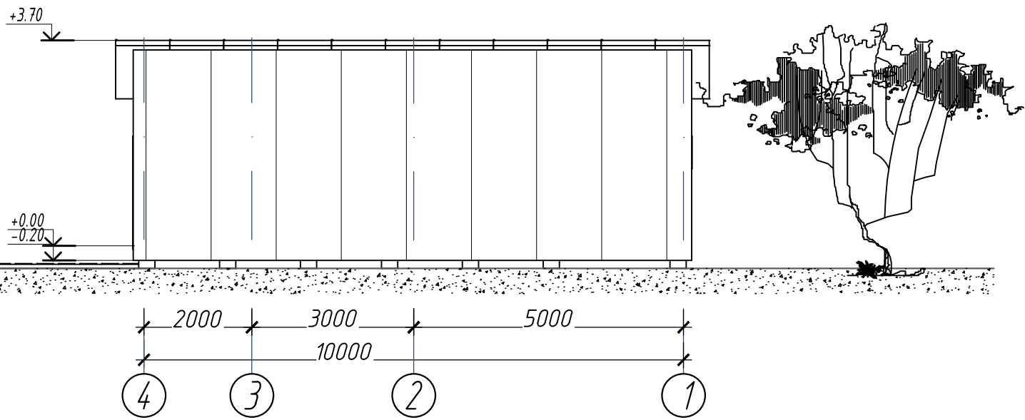
Fatada 4-1
