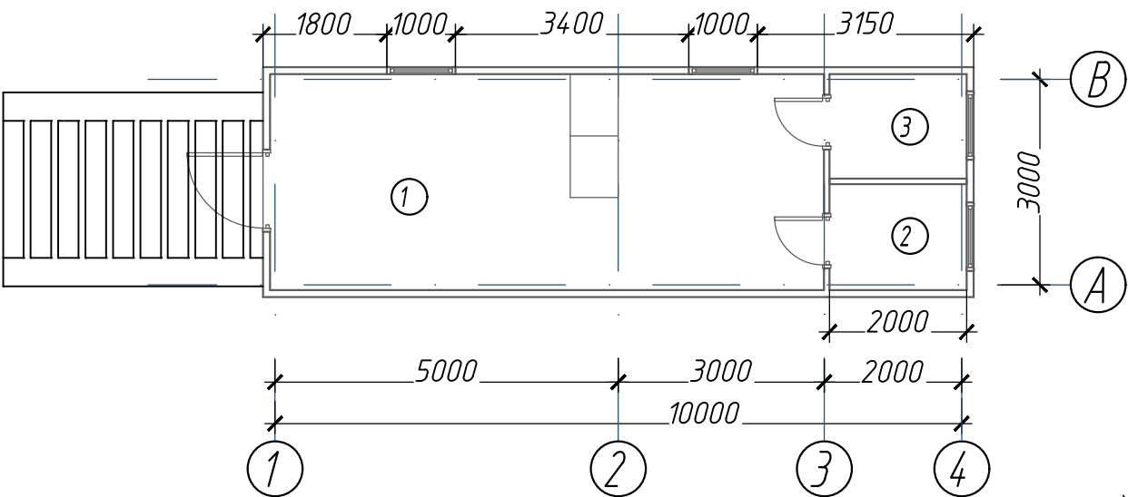
Plan parter, cota: 0.000
