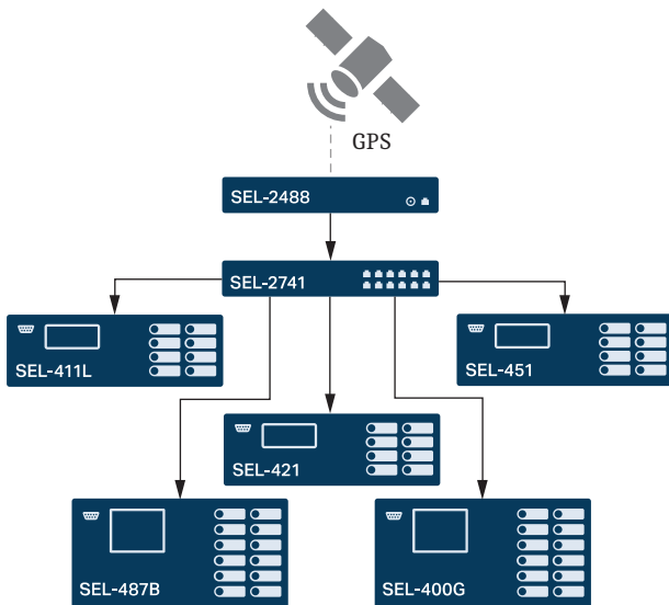
Figure 28 Example PTP Network
