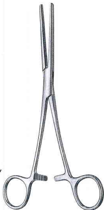
Rochester-Pean
