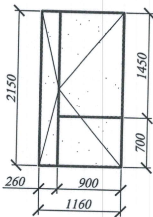
Usi 651,652,655,656-4buc
