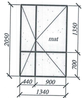
Usi 638,639-2buc
