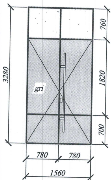
Usa intrare in bloc-1buc
