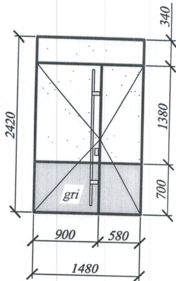
Usa intrare in bloc-1buc
