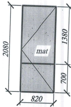
Usi 630,631,-2buc
