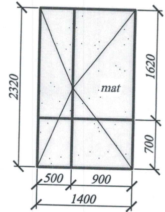
Usi 623,624A,629-3buc
