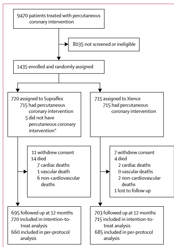
Figure 1: Study profile
