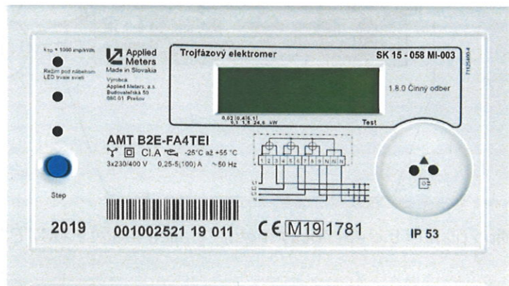
Fig. 3b: Example of marking directly on cover of the electricity meter – Applied Meters AMT B2x-FA4T9I(E) (alternative - by laser printing)
