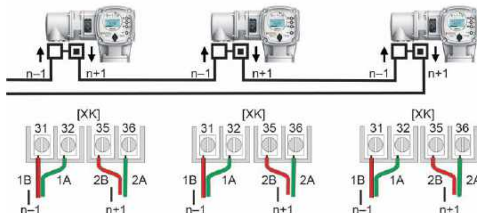
Figure 24: Terminal assignment for loop topology (2-channel)
