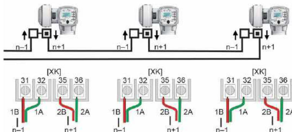
Figure 39: Terminal assignment for loop topology (2-channel)
