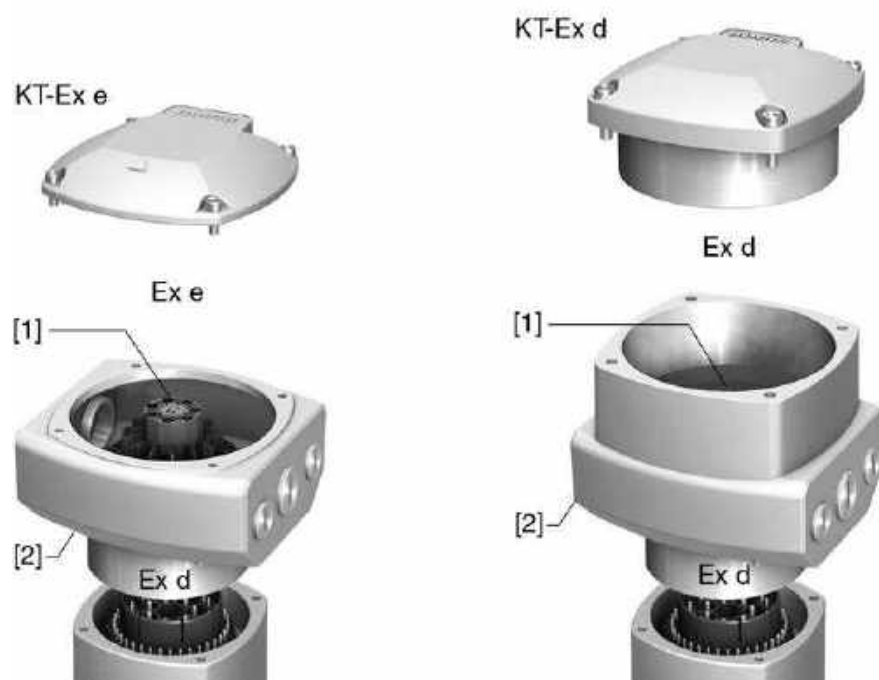
Figure 24: KT/KM electrical connection
