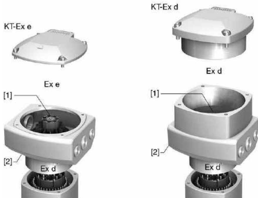
Figure 33: KT/KM electrical connection
