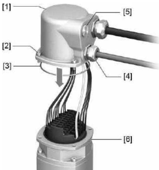
Figure 18: Close terminal compartment
