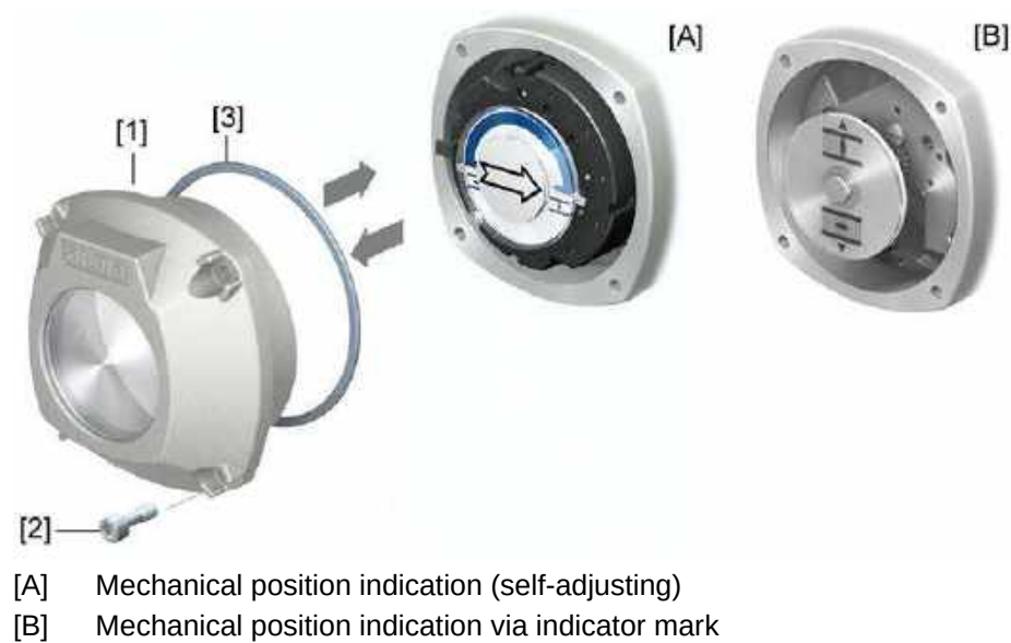
Figure 81: Open/close switch compartment
