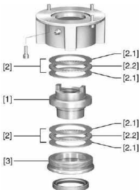
Figure 11: Output drive type A
