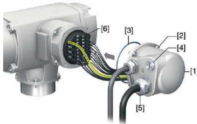
Figure 25: Close terminal compartment
