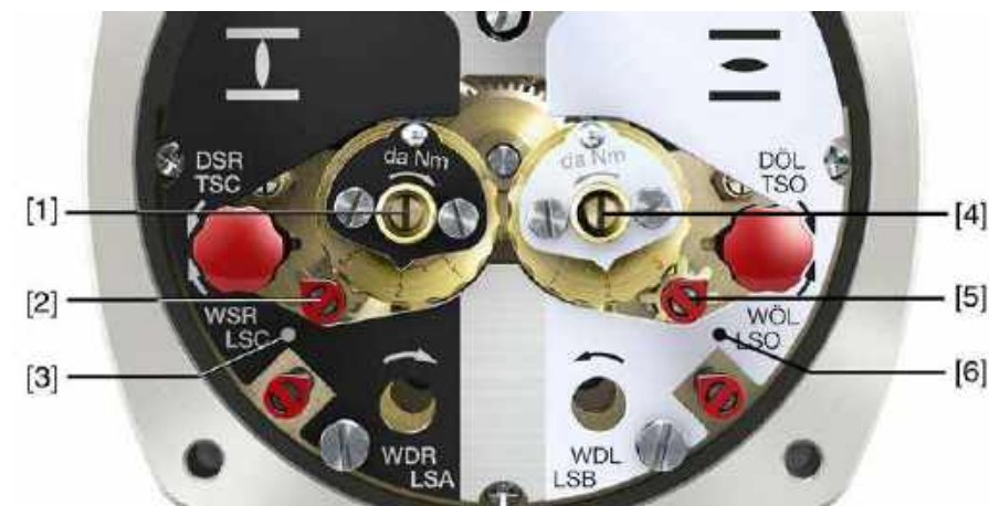
Figure 35: Setting elements for limit switching
