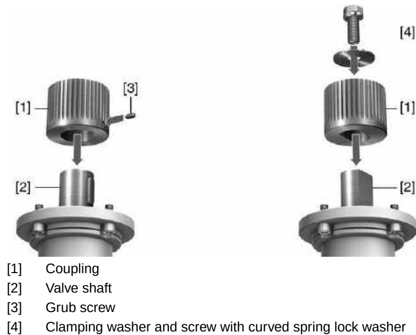
Figure 11: Mounting positions for coupling
