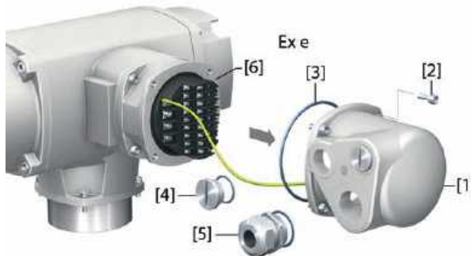
Figure 20: Open terminal compartment
