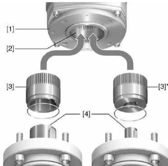
Figure 13: Output drive type B
