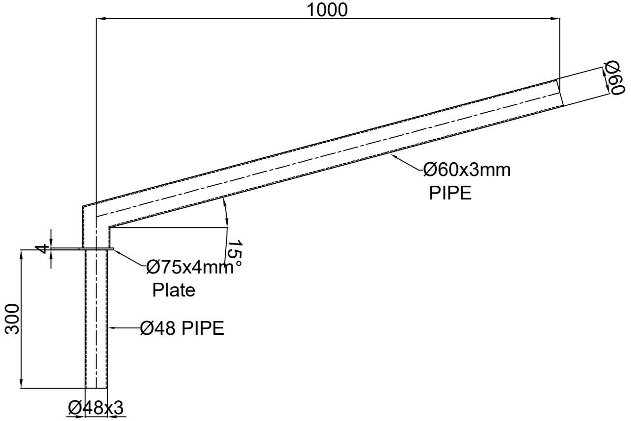
SINGLE BRACKET ARM DETAIL
