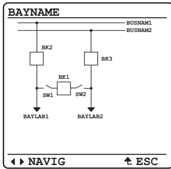
Figure 9 Breaker-and-a-Half
