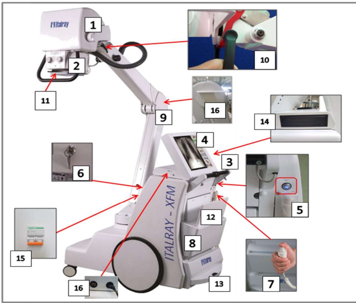
Figura 1 System composition
