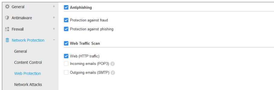
Computers and Virtual Machines Policies - Network Protection - Web Protection
