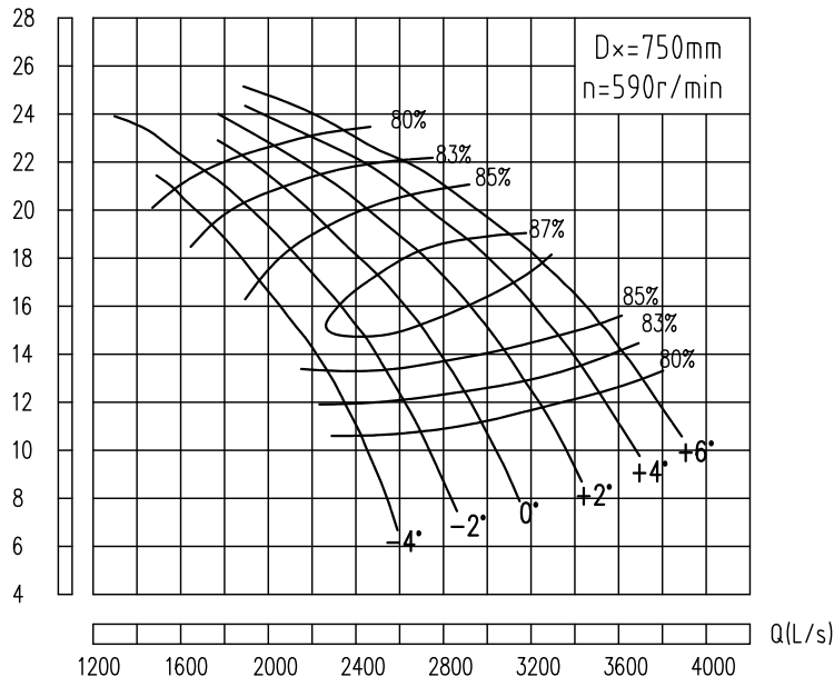
H(m) 900HLB-40
