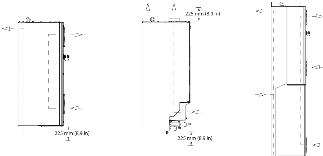
Illustration 5.18 Optional Airflow Configuration Using Back-channel Cooling Kits for Enclosures D1h–D8h.
