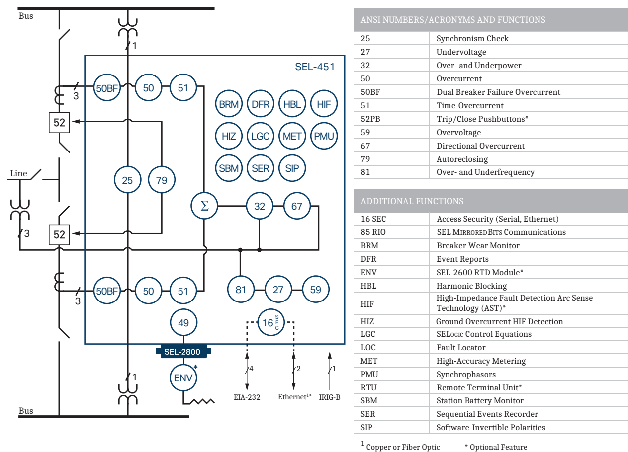
Figure 1 Functional Overview
