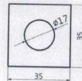
Square Flat Washer 35x35x5
